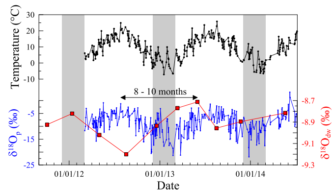
Fig. 10. Relationship between \delta^{18}O in precipitation at Mormont station and in M6 drip water. Temperatures at Fahy station are shown in the upper panel. Winter seasons (DJF) are highlighted in grey.
